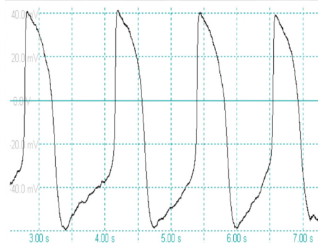
HIPS cardiomyocyte action potentials recorded with the Patchserver
